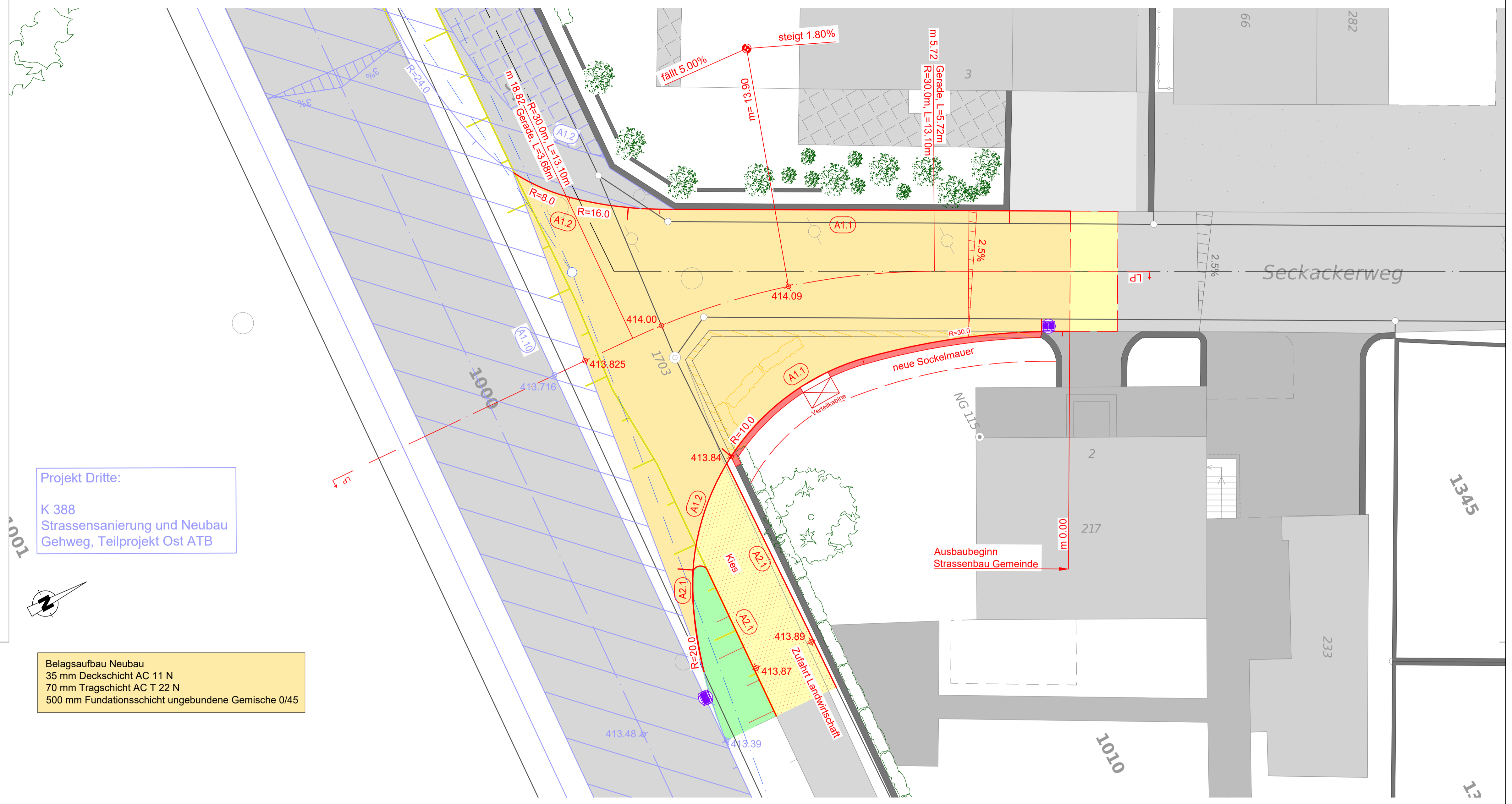
Situation 1:100
